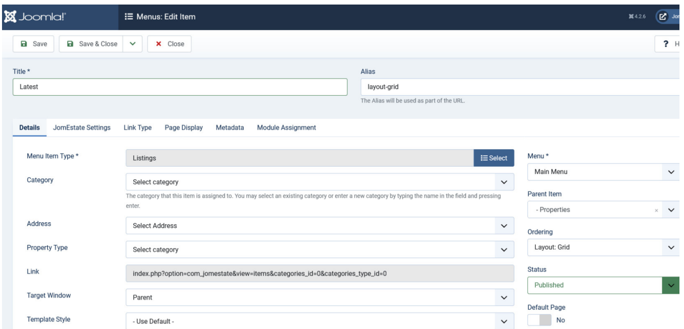
Screen 3: Items menu item screen
